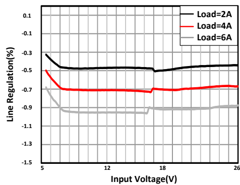
Figure 11-6. Line Regulation
