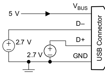
Figure 10-22. Divider 3 Mode
