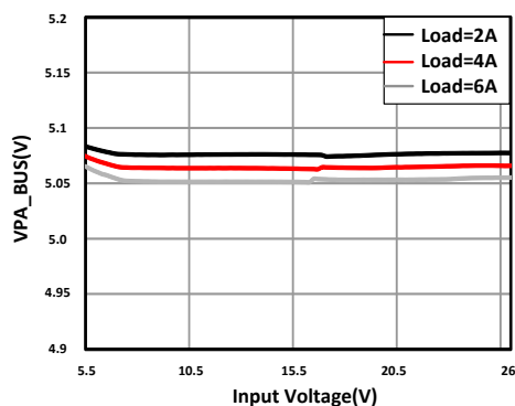
Figure 11-12. Dropout Characteristic
