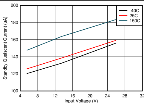
Figure 8-2. Standby Quiescent Current
