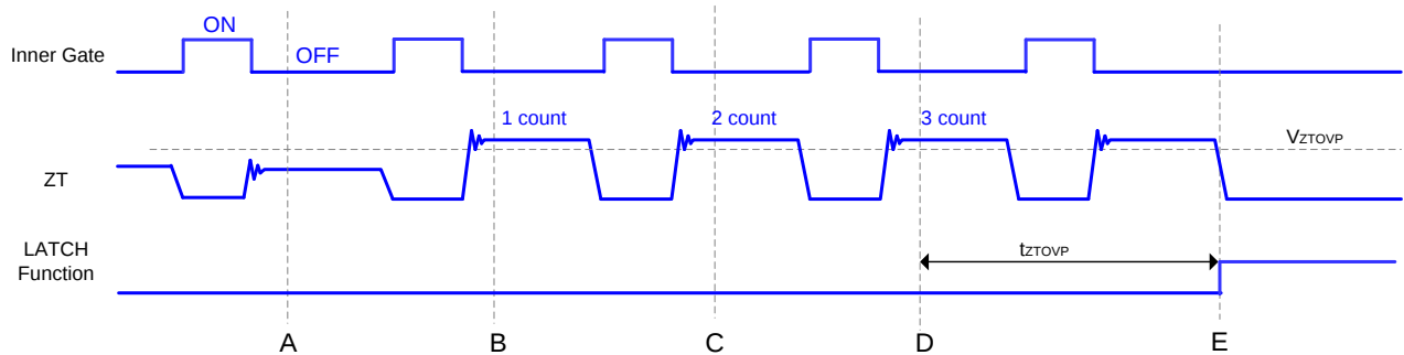
Figure 10. ZT pin over voltage protection (Pulse detection)
