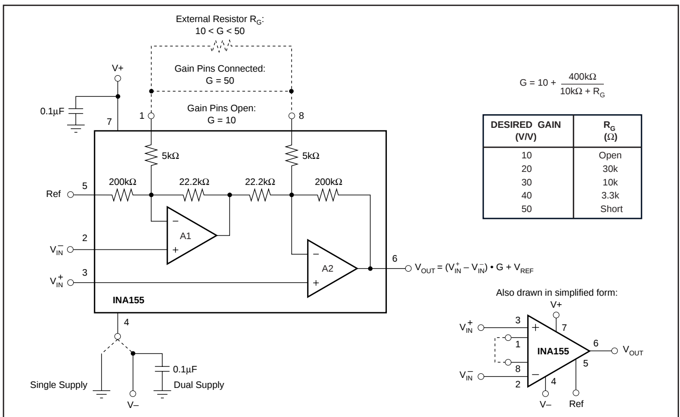
FIGURE 1. Basic Connections.
