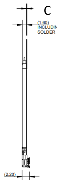
Side View
