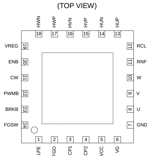
Figure 2. Pin Configuration
