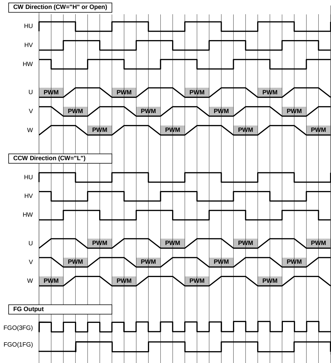
Figure 4. Timing Chart
