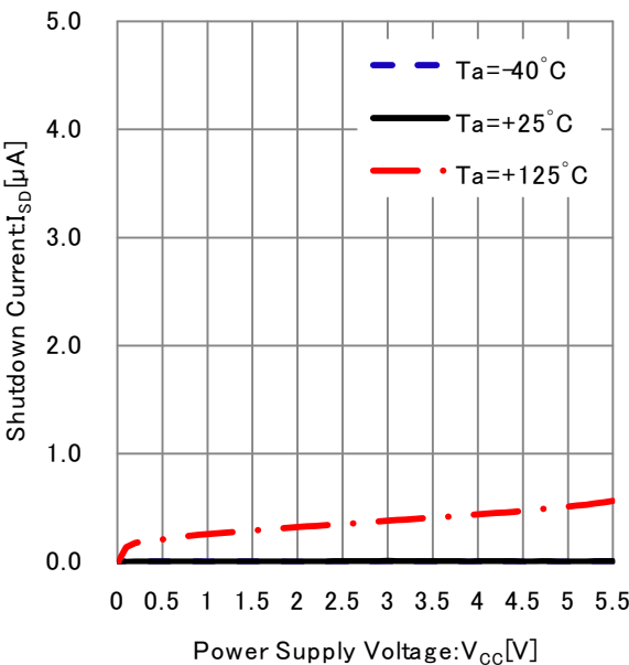
Figure 27. Shutdown Current vs Power Supply Voltage
