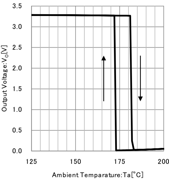
Figure 29. Output Voltage vs Ambient Temperature
