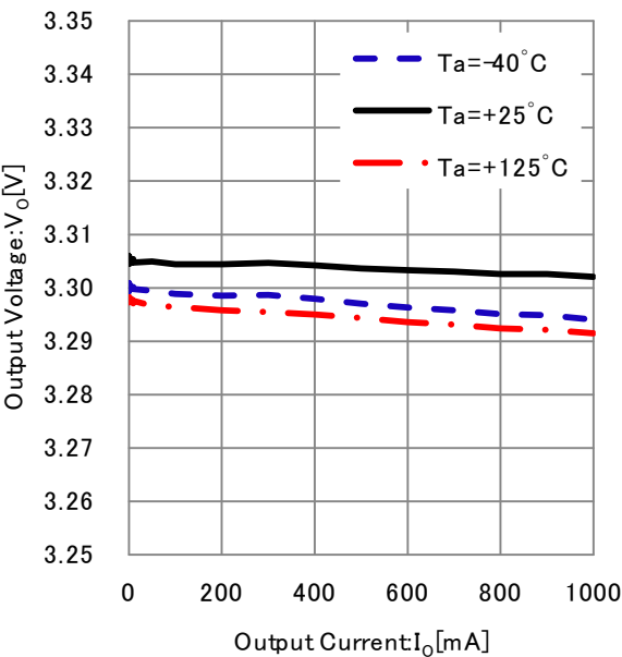
Figure 26. Output Voltage vs Output Current
