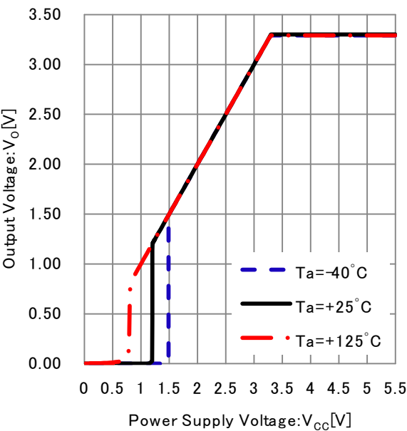
Figure 28. Output Voltage vs Power Supply Voltage
