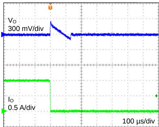
Figure 8. Transient Response (1000 mA→1 mA, T_a = +25\text{ }^\circ\text{C} )
