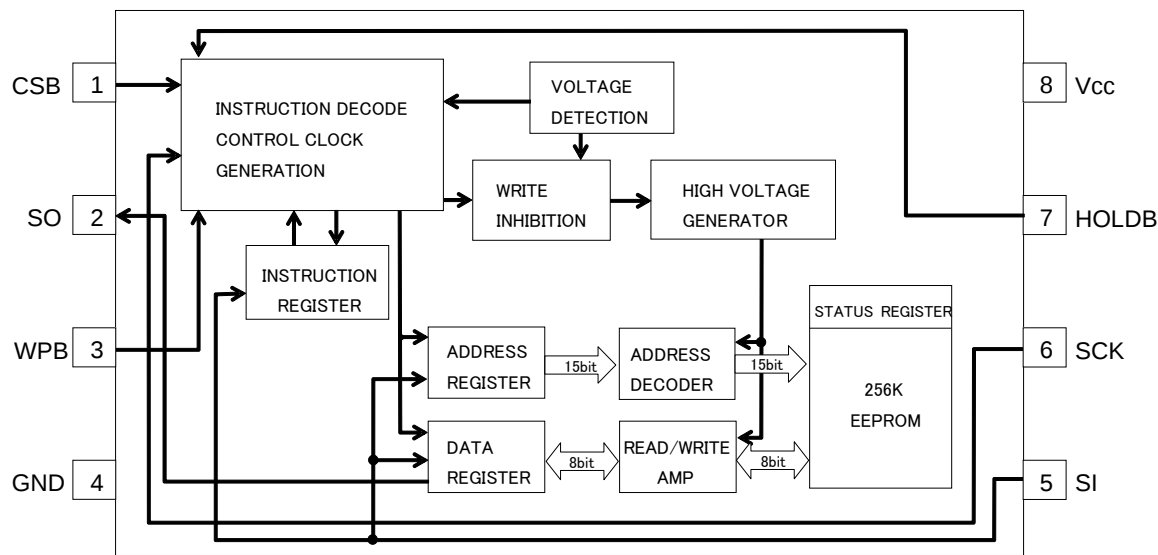
Figure 3. Block Diagram
