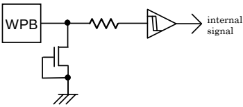
Figure 57. WPB input equivalent circuit
