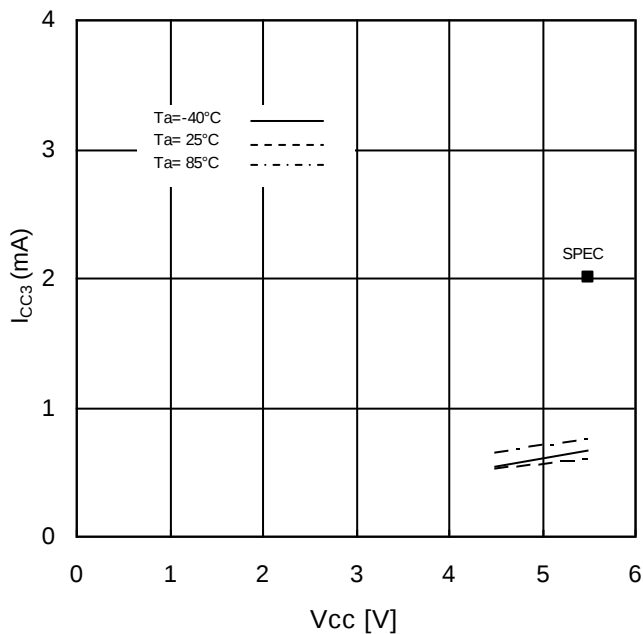
Figure 15. Supply Current (Write) vs Supply Voltage ( f_{SCK}=20\text{MHz} )
