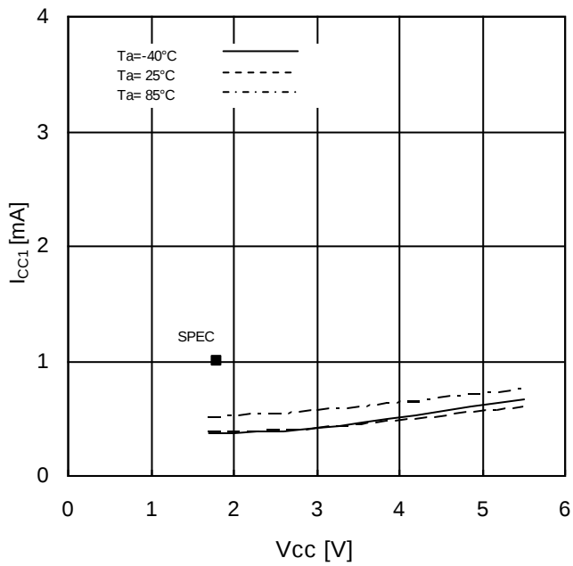
Figure 13. Supply Current (Write) vs Supply Voltage ( f_{SCK}=5\text{MHz} )
