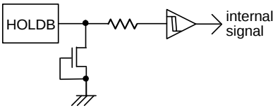
Figure 56. HOLDB input equivalent circuit
