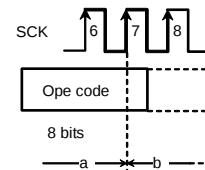
Figure 48. WREN/WRDI cancel valid timing
