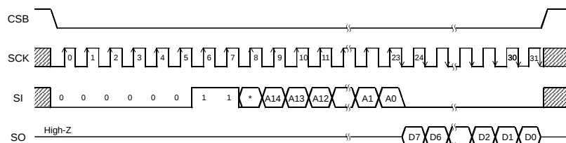
Figure 39. Read command
