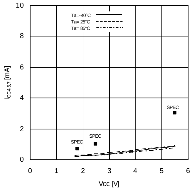
Figure 16. Supply Current (Read) vs Supply Voltage ( f_{SCK}=5\text{MHz} )
