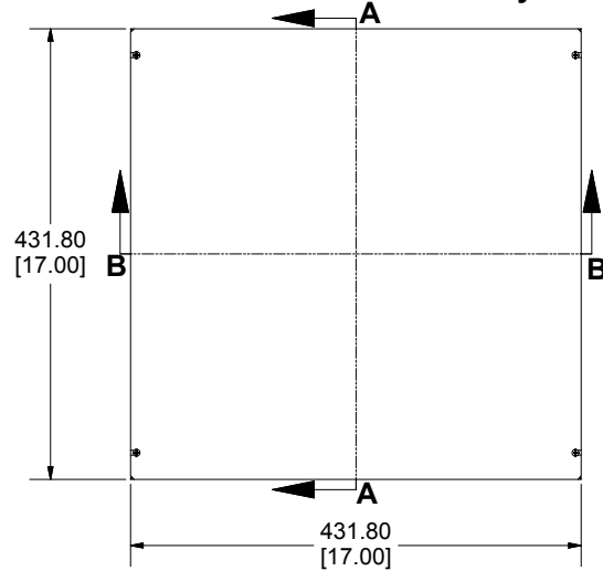
Bottom View of Assembly
