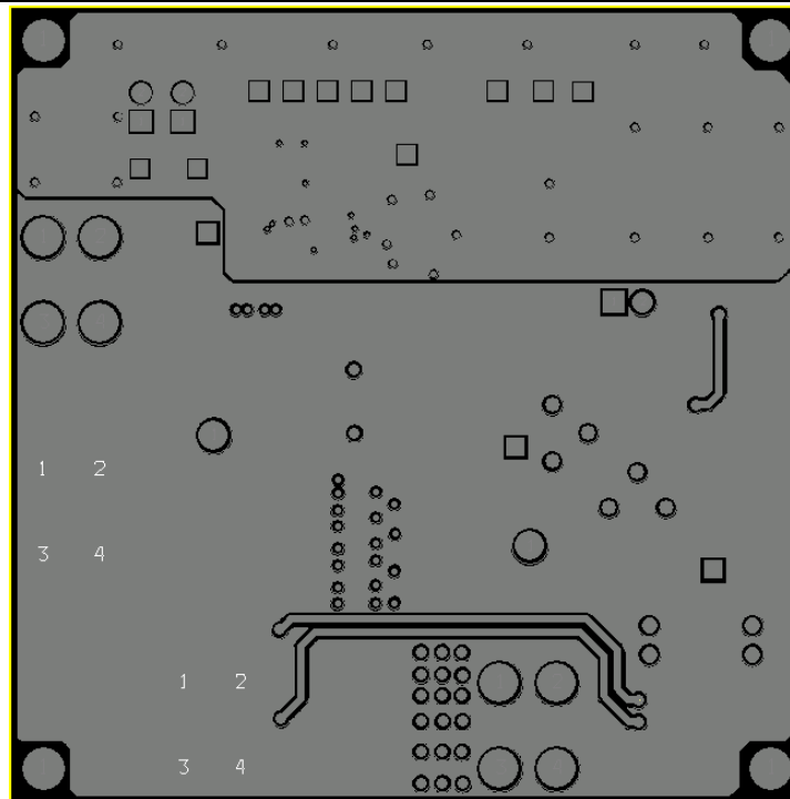
Figure 9. Inner Layer 1
