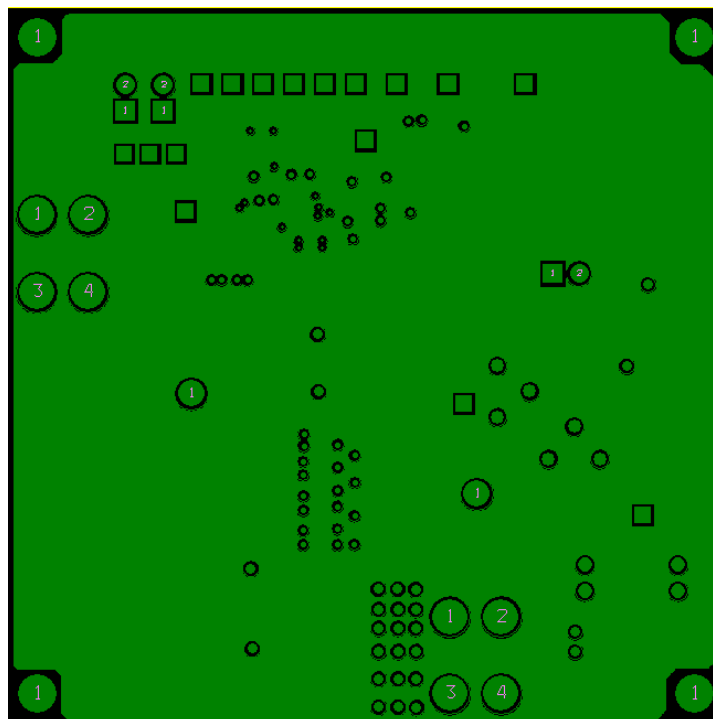
Figure 10. Inner Layer 2
