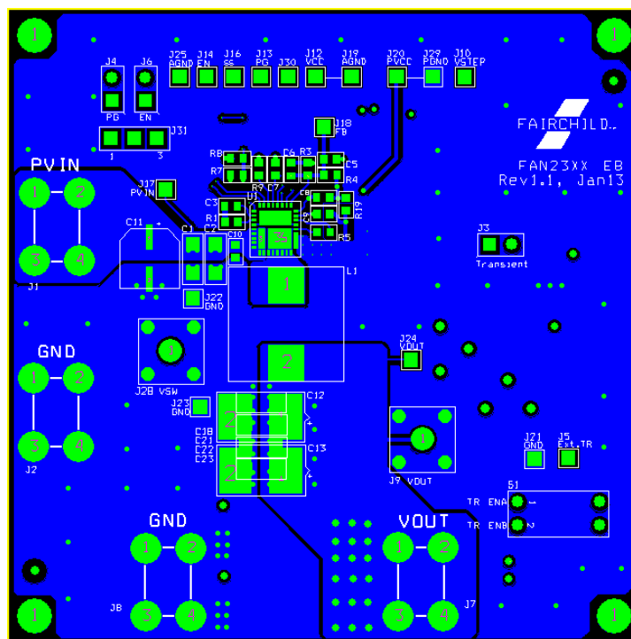
Figure 7. Top Side
