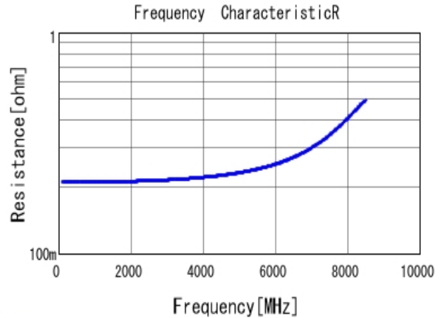
■ GCQ1555C1H1R6WB01 R DC0V, 25degC
