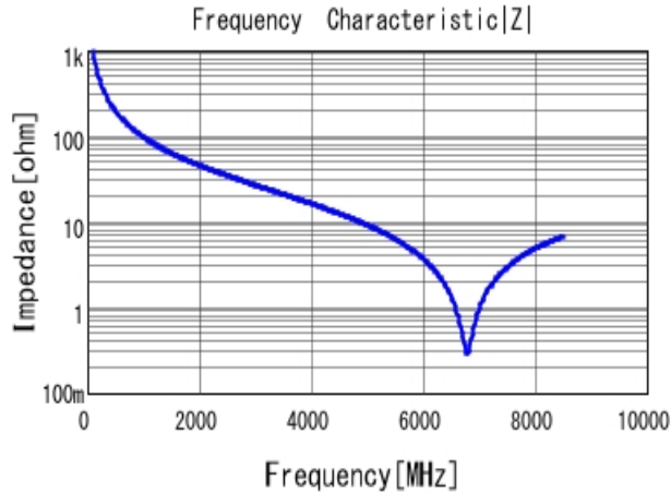
■ GCQ1555C1H1R6WB01 |Z| DC0V, 25degC
