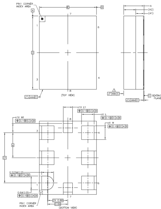
Figure 6.3. Si549 (2.5x3.2 mm) Outline Diagram
