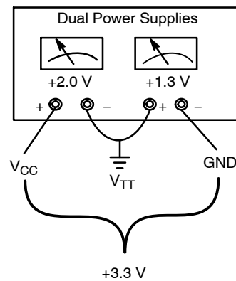
Figure 3. “Split” Power Supply Connections
