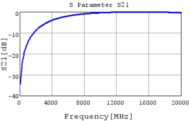
GCQ1555C1HR30WB01 S21 DCOV, 25degC
