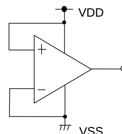
Figure 27. Example of Application Circuit for Unused Comparator
