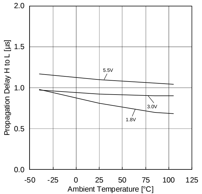
Figure 22. Propagation Delay H to L vs Ambient Temperature ( C_L=15\text{pF} , I_N=-1.5\text{V} 100mV Overdrive)
