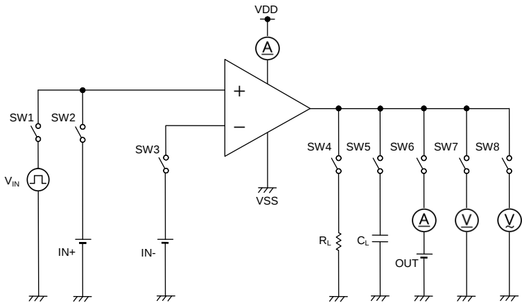
Figure 24. Test Circuit 2
