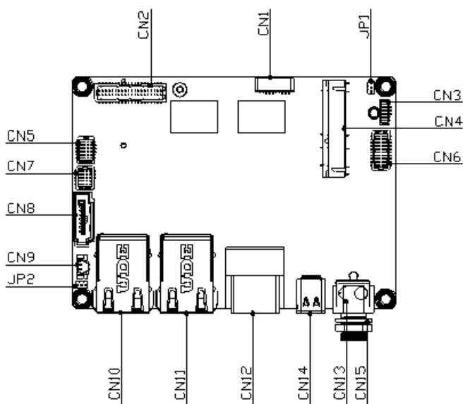
Component Side
