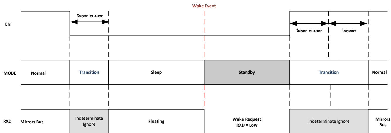
Figure 8-14. Mode Transitions
