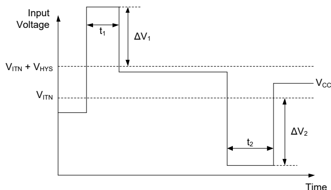
Figure 9. Overdrive Voltage
