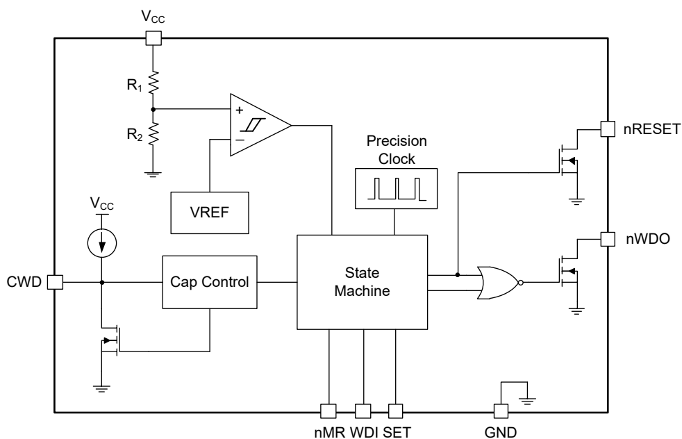
Figure 4. SGM820 Block Diagram
