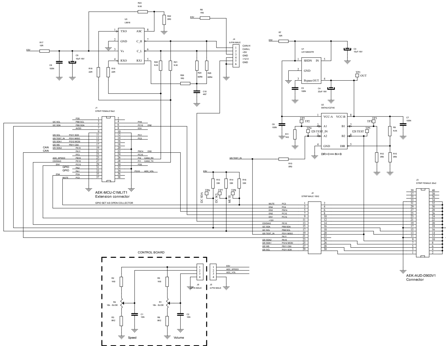
Figure 3. Schematic diagram
