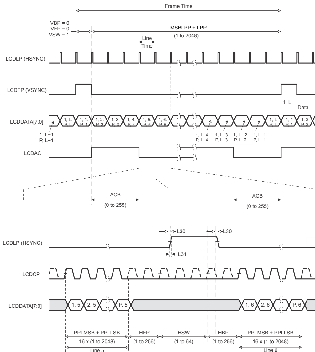
Figure 28-54. LCD Raster-Mode Passive
