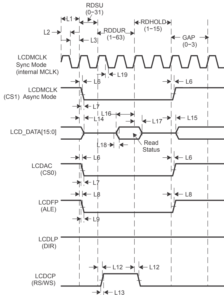
Figure 28-48. Motorola 6800 Graphic Display Mode Status (Synchronous & Asynchronous Operation)
