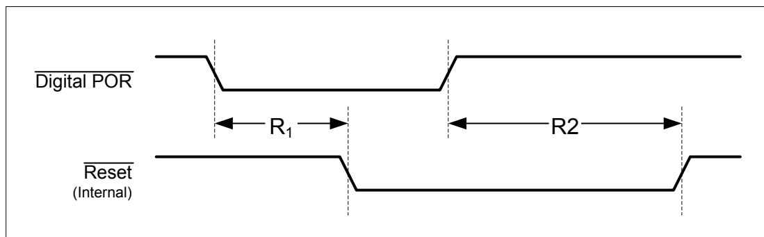
Figure 28-9. Digital Power-On Reset Timing
