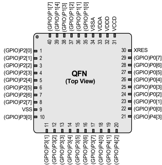
Figure 9. 40-Pin QFN Pinout
