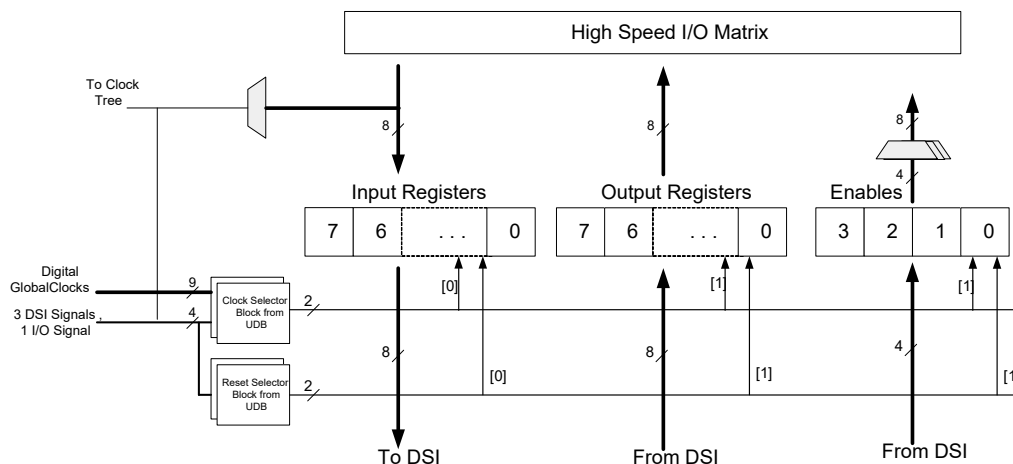
Figure 6. Port Interface
