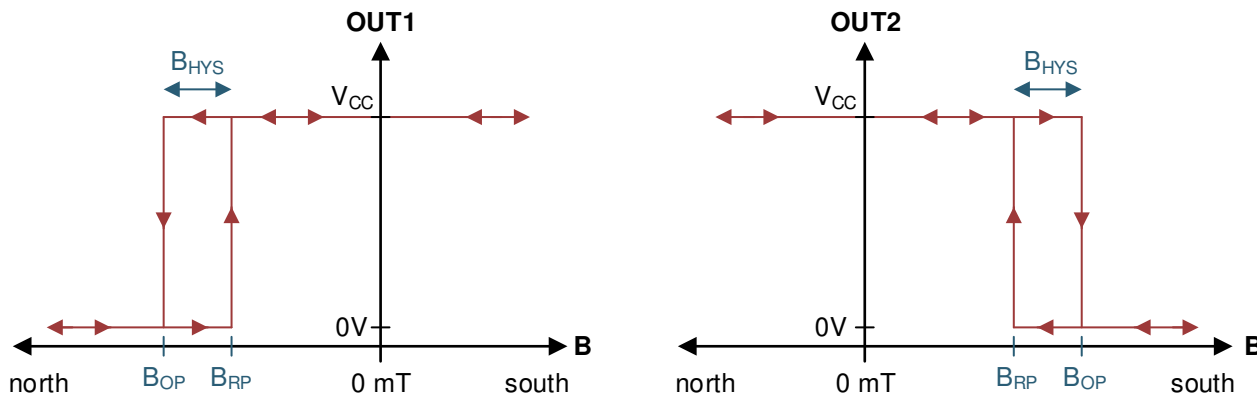
Figure 8-4. Unipolar Functionality
