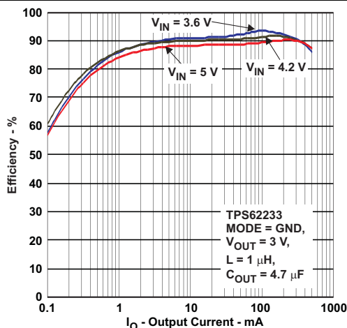
Figure 32. Efficiency vs I_{O} – TPS62233
