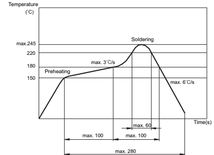
RECOMMENDED REFLOW SOLDERING PROFILE (For SMT type, for applications with PCB thickness \leq 3\text{mm} ) 7)
