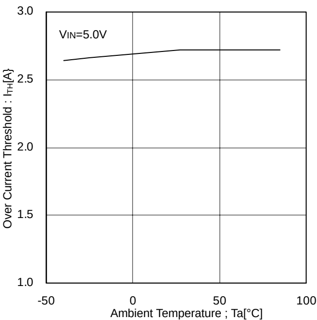
Figure 15. Over-Current Threshold
