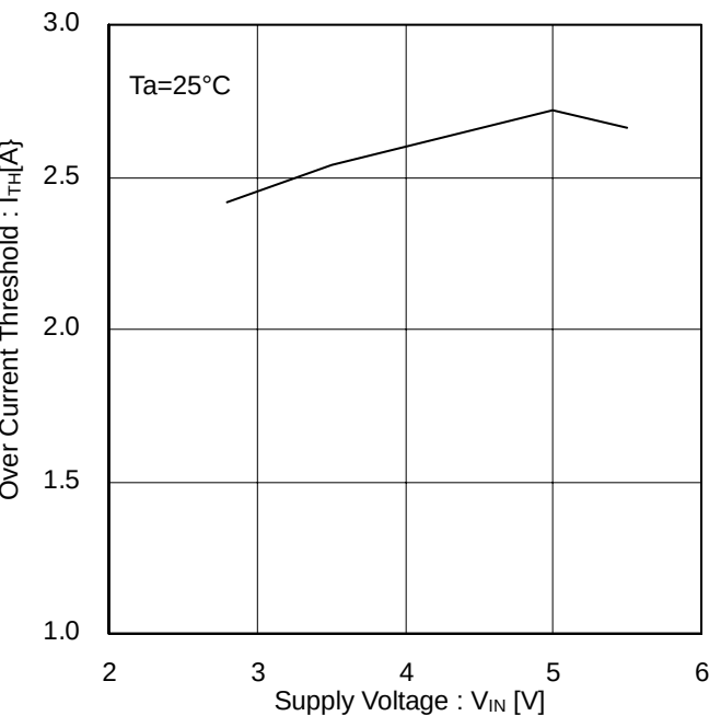
Figure 14. Over-Current Threshold
