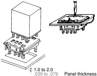
Panel cutout for tandem mounting
