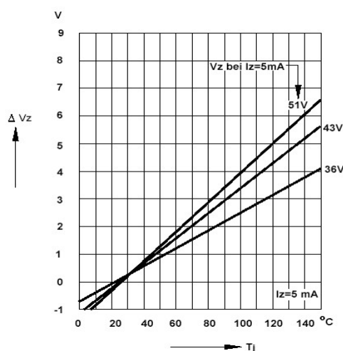
Figure 14. Change of Zener Voltage vs. T j
