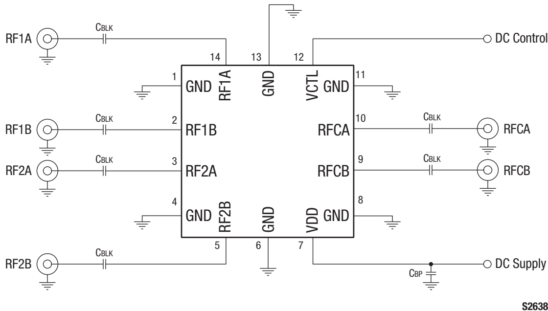
Figure 7. SKY13421-486LF Evaluation Board Schematic
