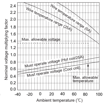
Operating range
