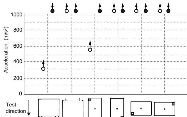
Shock resistance characteristics
