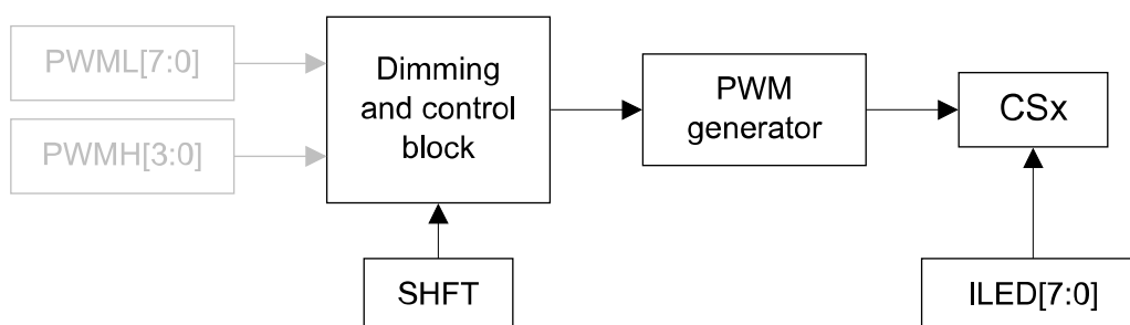
Figure 5. Analog dimming
