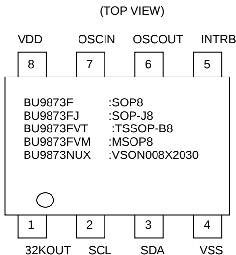
Figure 3. Pin configuration
