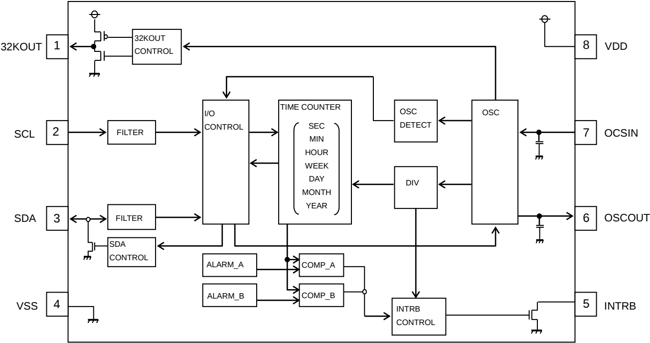
Figure 4. Block diagram
