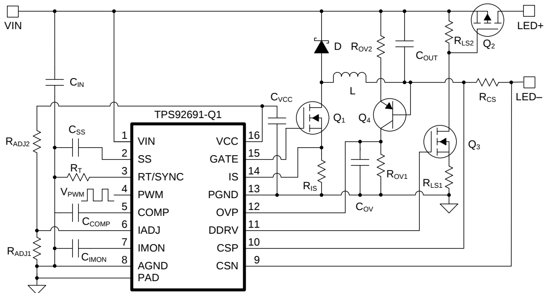
Figure 27. Buck LED Driver
