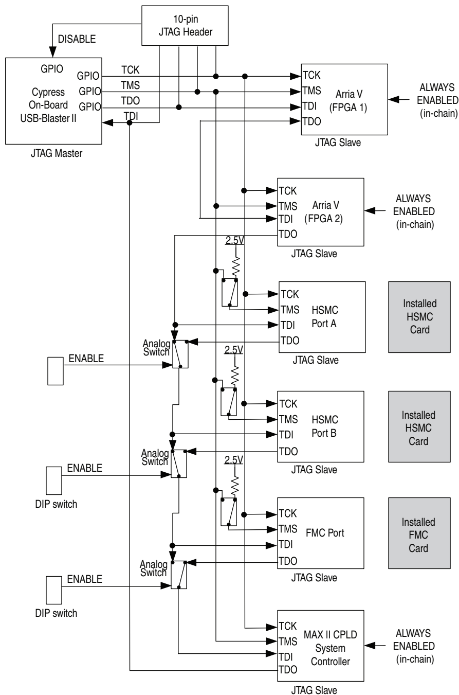
Figure 2-4. JTAG Chain
