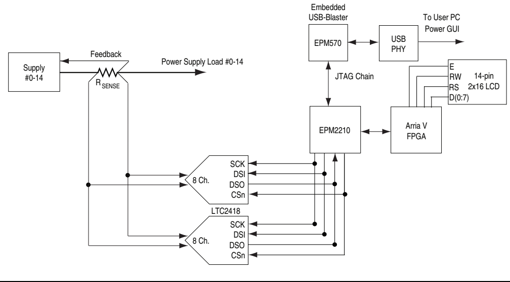
Figure 2-13. Power Measurement Circuit
