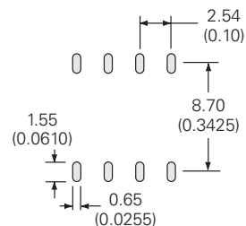
PCB Land Pattern
