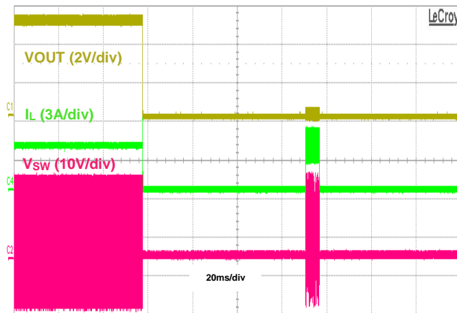
Figure 47. Output Short Protection, I_{OUT} = 3.5\text{A}
