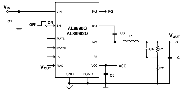
Figure 1. Typical Application Circuit for Constant Voltage Output
