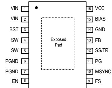
TSSOP-16EP (Top View)
