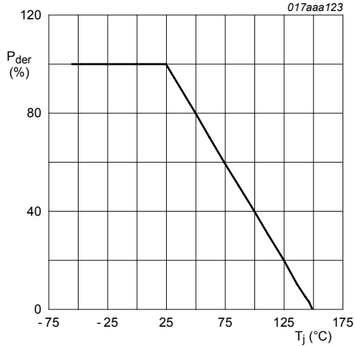
Fig. 2. Normalized total power dissipation as a function of junction temperature
