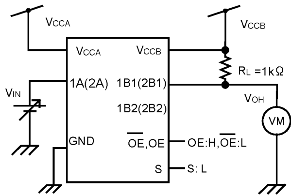
Fig. 15.1 Test Circuit
