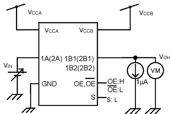
Fig. 16.1 Test Circuit
