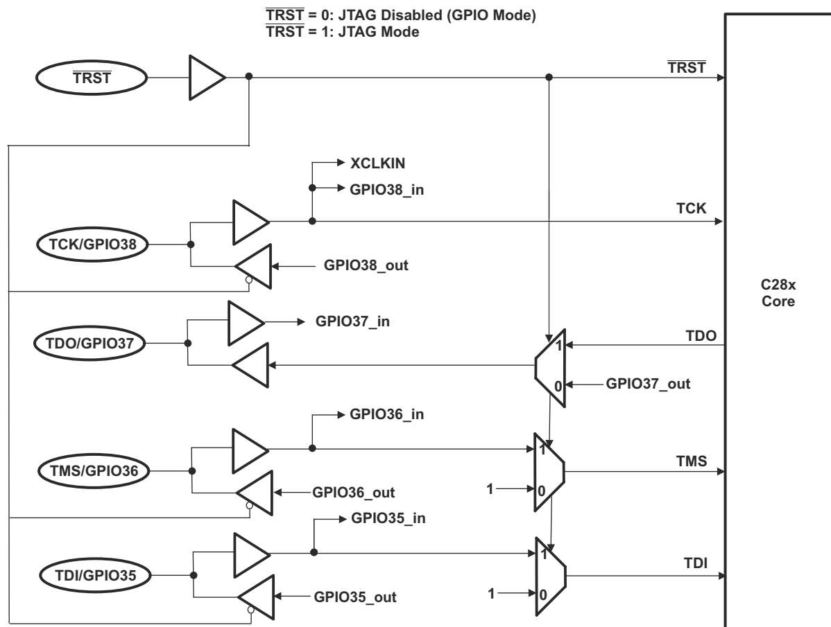
Figure 7-44. JTAG/GPIO Multiplexing
