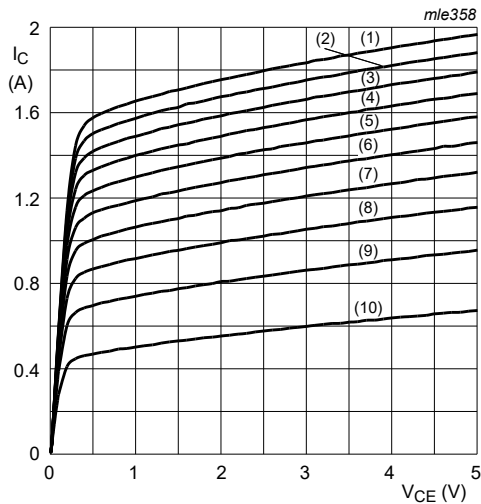
T_{amb} = 25^\circ\text{C} (1) I_B = 3500\ \mu\text{A} (2) I_B = 3150\ \mu\text{A} (3) I_B = 2800\ \mu\text{A} (4) I_B = 2450\ \mu\text{A} (5) I_B = 2100\ \mu\text{A} (6) I_B = 1750\ \mu\text{A} (7) I_B = 1400\ \mu\text{A} (8) I_B = 1050\ \mu\text{A} (9) I_B = 700\ \mu\text{A} (10) I_B = 350\ \mu\text{A}
