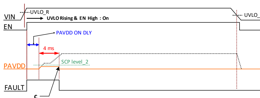
Figure 11. SCP Mechanism When PAVDD Pre-Charge Under Abnormal Heavy Load Conditions
