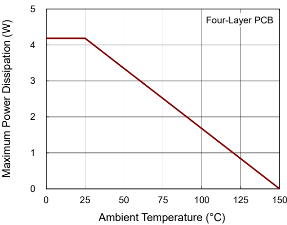
Figure 19. Derating Curve of Maximum Power Dissipation
