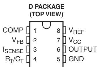
Figure 5-1. SOIC Package 8-Pin D Top View
