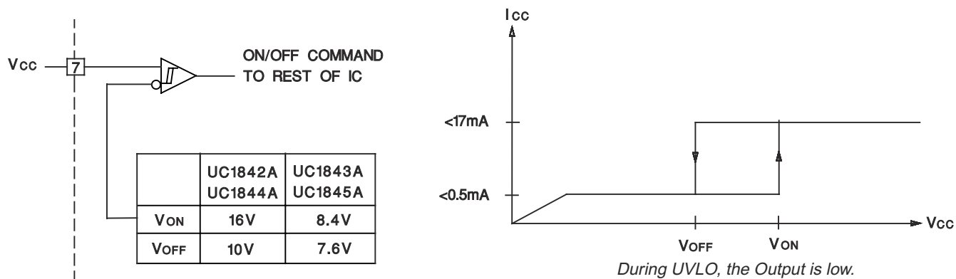
Figure 7-3. Undervoltage Lockout
