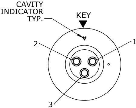
WIRE VIEW W17280-3PG-P-300
