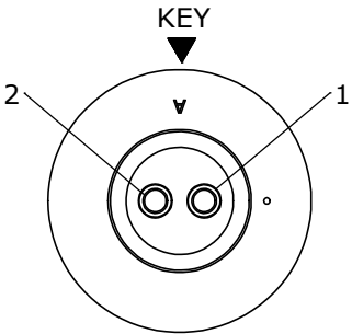
WIRE VIEW W17280-2PG-P-300
