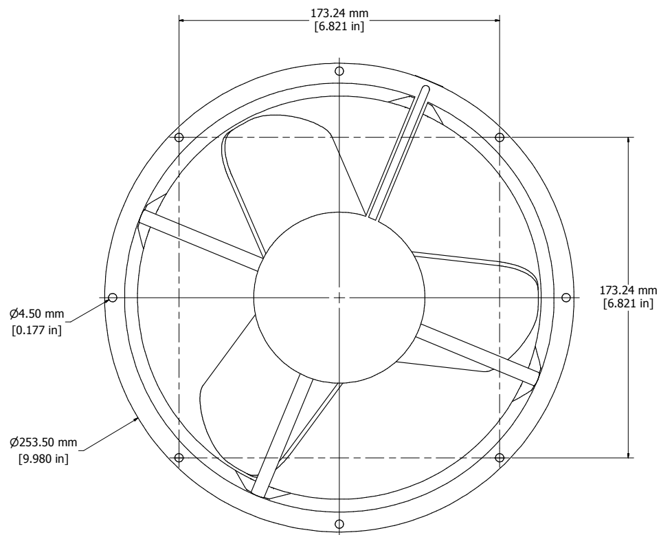
TOP VIEW
