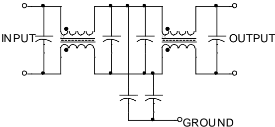
Figure 4. Internal Schematic
