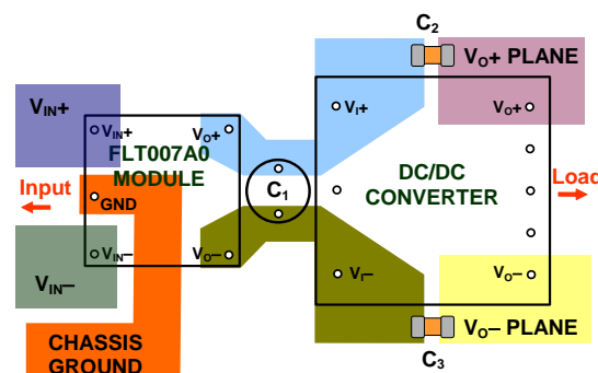
Figure 6. Diagram showing recommended layout of the FLT007A0Z filter module with open-frame DC/DC converter modules.
