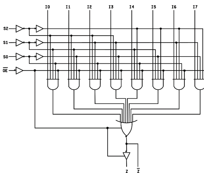
FIGURE 3. Logic diagram.
