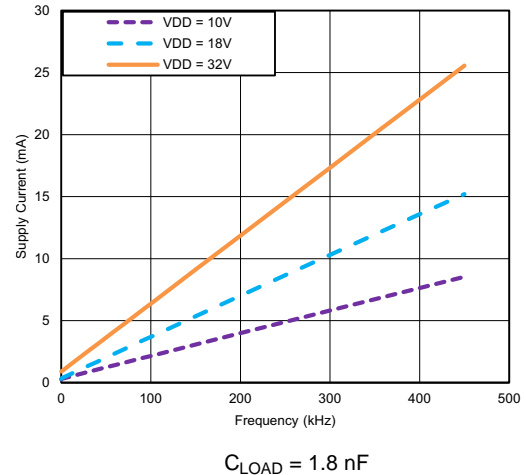
Figure 9. Operating Supply Current vs. Frequency
