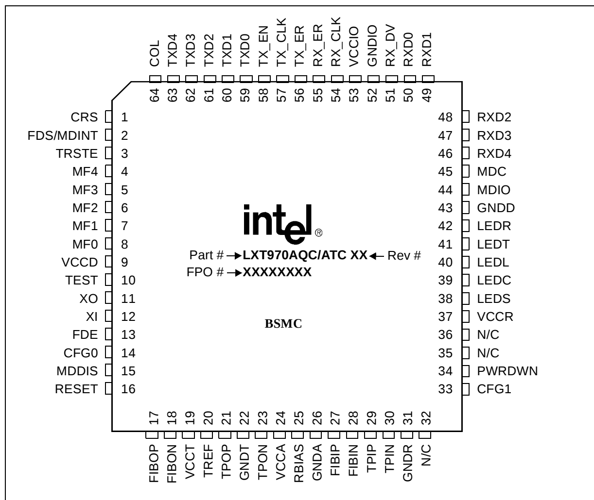
Figure 2. Pin Assignments
