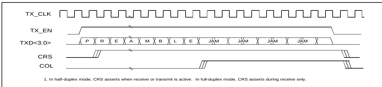
Figure 19. 00BASE-TX Transmission with Collision
