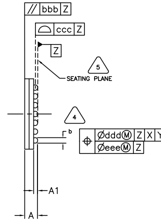
Figure 18. 50-Ball WFBGA Mechanical Drawing
