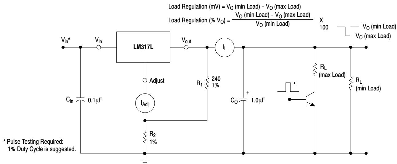
Figure 3. Load Regulation and \Delta I_{Adj}/\text{Load} Test Circuit
