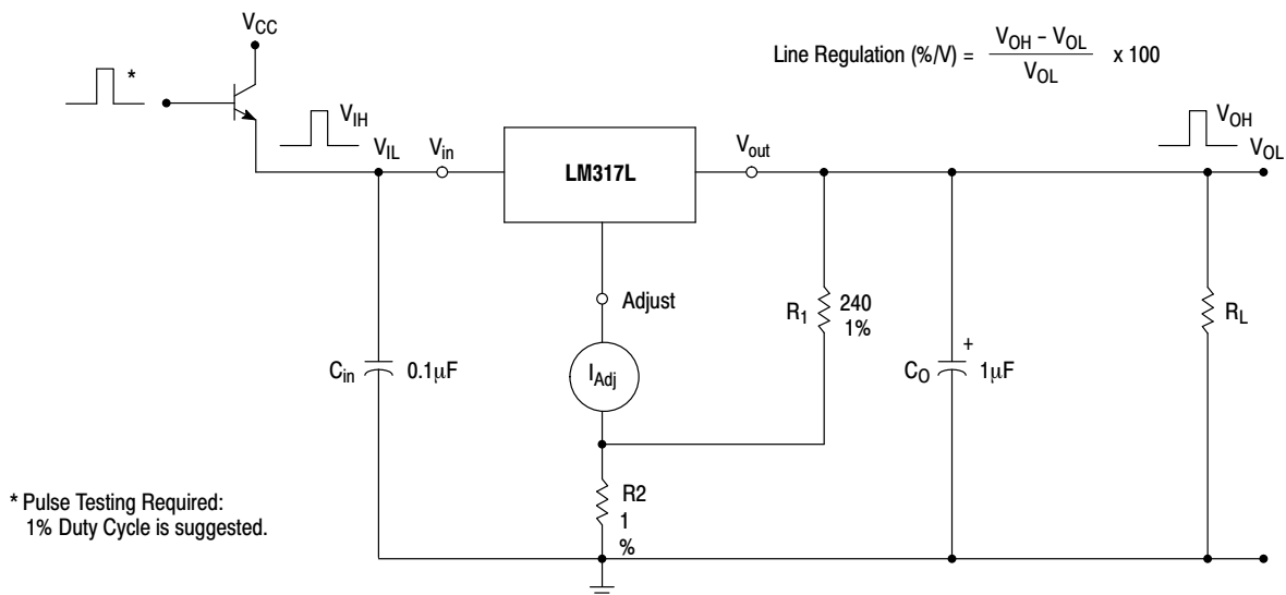
Figure 2. Line Regulation and \Delta I_{Adj}/Line Test Circuit
