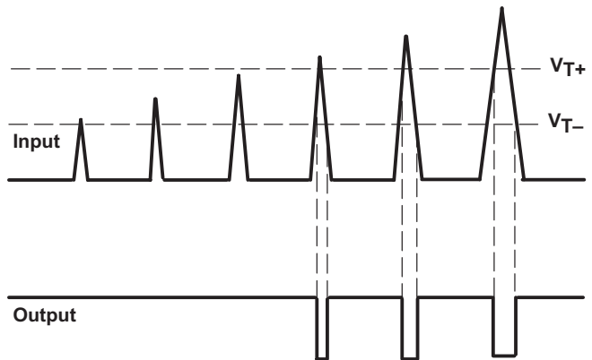
Figure 34. Pulse Stretcher
