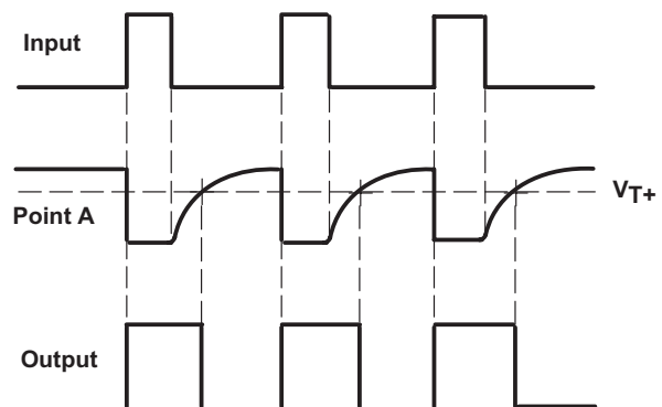
Figure 33. Threshold Detector
