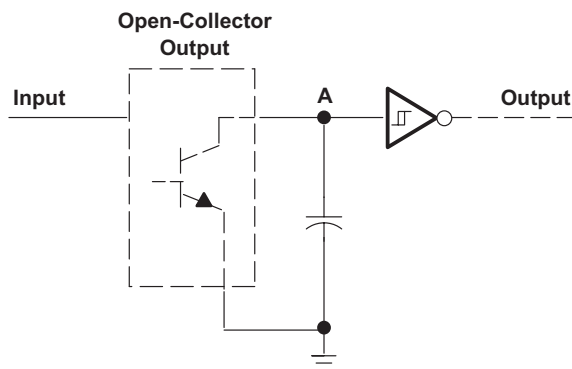
Figure 33. Threshold Detector
