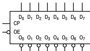
Figure 2. Logic Symbol
